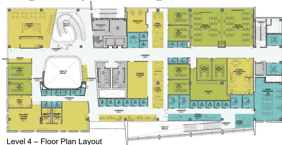
Level 4 – Floor Plan Layout
